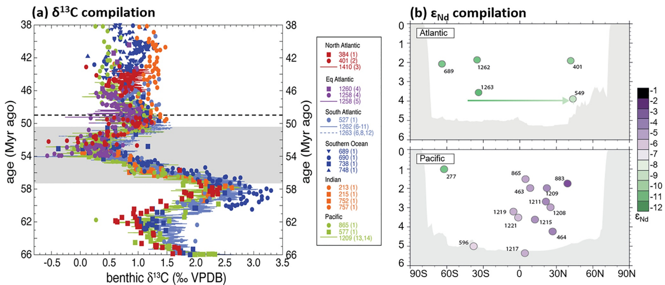
Figure 7. Proxy-based ocean circulation. (a) Deep sea (benthic foraminifera) \delta^{13}\text{C} compilation through the Palaeocene and Eocene from deep-sea drilling sites (~1,500–3,500 m paleo-water depth), grouped by geographical region (ocean basin). Gray shaded bar denotes interval of diminished benthic \delta^{13}\text{C} differences between ocean basins, that approximately corresponds to the early Eocene. Dashed line marks the timing of onset of the progressive Cenozoic global cooling trend. Ages for all data sets are converted to the new calibration of the geomagnetic polarity timescale (Westerhold et al., 2020). Data sources numbered in the figure legend are: (1) Zachos (2001), (2) Bornemann et al. (2016), (3) Vahlenkamp et al. (2018), (4) Sexton et al. (2006), (5) Sexton et al. (2011), (6) Laurentano et al. (2015), (7) Littler et al. (2014), (8) Stap et al. (2010), (9) McCarren et al. (2008), (10) Barnett et al. (2019), (11) Barnett et al. (2018), (12) Laurentano et al. (2016), (13) Westerhold et al. (2018), and (14) Westerhold et al. (2011). (b), compilation of neodymium (Nd) isotope signatures as a function of depth and latitude covering the time window from 54 to 45 Ma in the Atlantic (omitting marginal sites 1001, 1258, and 1261) and Pacific (omitting marginal sites 1171 and 1172). Arrows indicate the potential direction of water-mass movement. Mean basin bathymetry from Herold et al. (2014).
