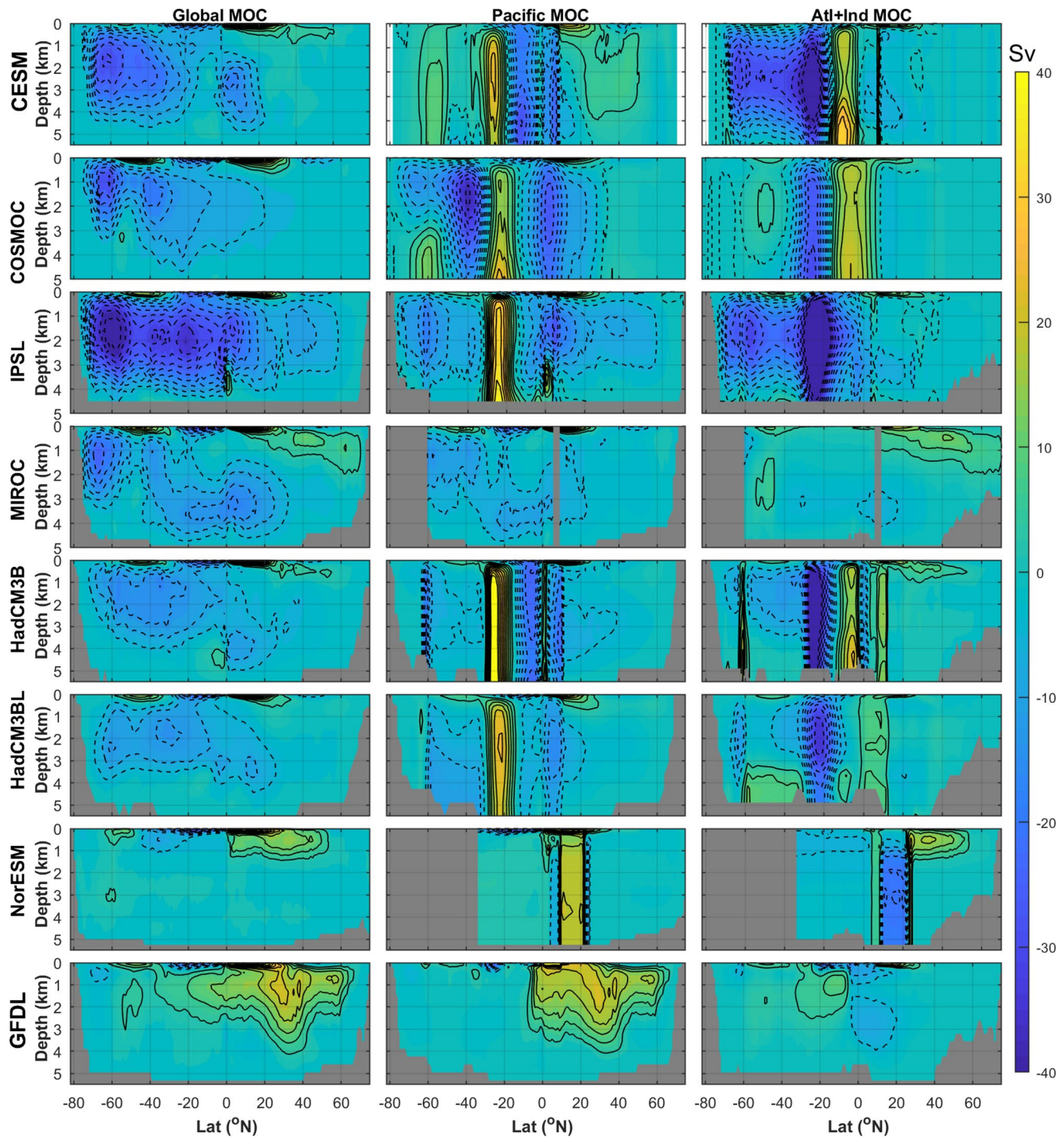
Figure 3. Separation of AMOC and PMOC from the global MOC in Eocene-3× simulations to show overturning circulation in two basins. Large values in the tropics indicate inter-basin exchanges, and a northward shift of these values in NorESM likely due to their more north tropical gateway that probably relates to their paleomagnetic reference bathymetry frame. NB, AMOC, and PMOC in the CESM, COSMOS, IPSL, and MIROC models are calculated offline.
